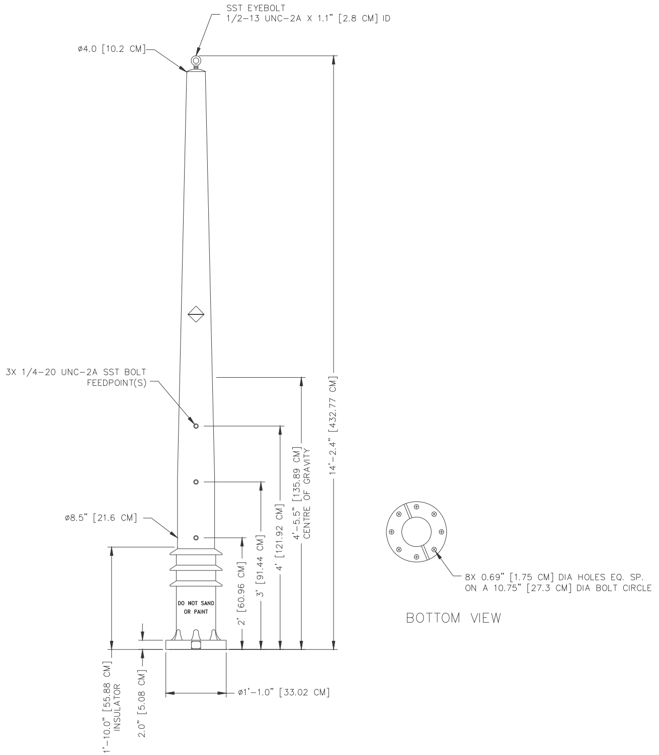
Figure 4-1 Outline Drawing
