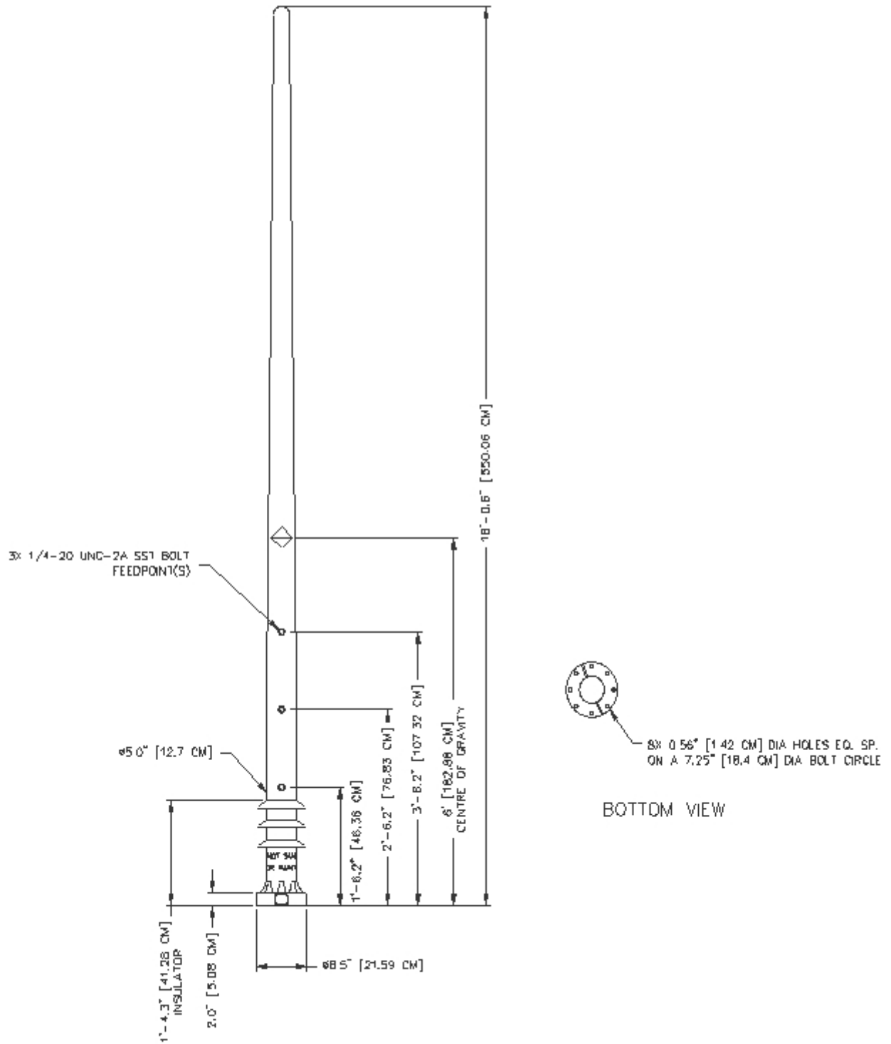
Figure 4-1 Outline Drawing
