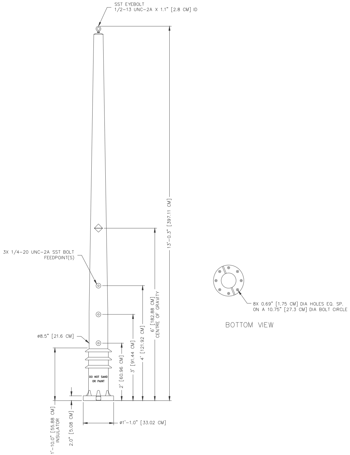
Figure 4-1 Outline Drawing
