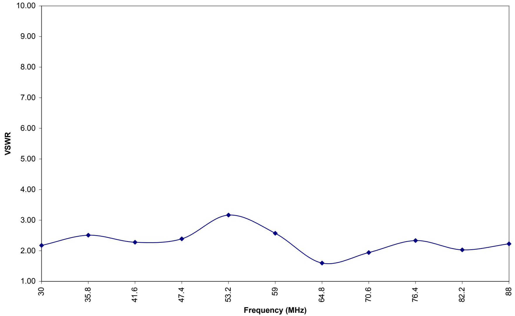
VSWR of AS-3900A/VRC from 30 MHz to 88 MHz
