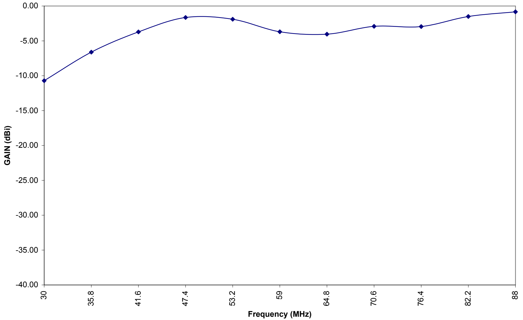
GAIN of AS-3900A/VRC from 30 MHz to 88 MHz
